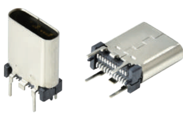
533 USB Type C Receptacle Vertical Height=6.5mm,9.3mm,10.5mm,12mm,15mm Positions:24
