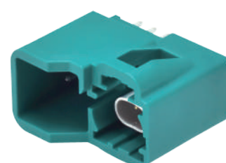
544 HMTD-N 1x1 +MQS 6Pin Vertical Type Coding: A,B,C,D,E,F,G,H,J,K,L,M,O,Z Positions: 06+02
