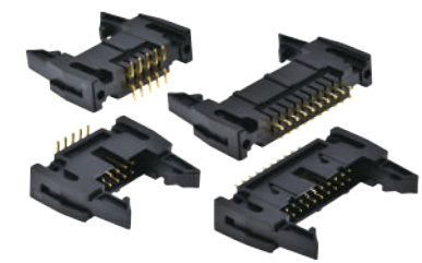
521 Ejector Header Pitch:2.54mm Positions:10,14,16,20,24,26,30,34,40,50,60,64
