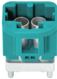
542 Mini FAKRA Plug 1x2 Vertical Type Coding:A,B,C,D,E,F,G,H,J,K,N,Z Positions:02
