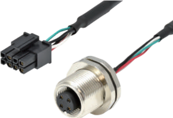
149 M12 A Code Female Rear/Front Mount, Free End Cable A Code Positions:04,05
