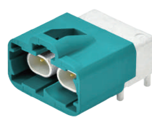
544 HMTD-N Plug 1x2 Right Angle Type Coding: A,B,C,D,E,F,G,H,J,K,L,M,O,Z Positions: 04
