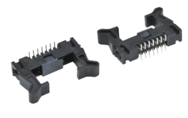
521 Ejector Header SMT Pitch:2.0mm Positions:6~64
