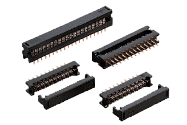
522 Transition Plug Pitch:2.54mm Positions:10,14,16,20,24,26,30,34,40,50,60,64
