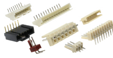
511 Wafer Pitch:0.8,1.0,1.25,2.0,2.54,3.0,3.96,4.25,5.08,6.35 Positions:02~40
