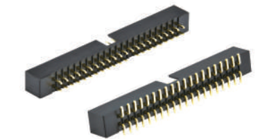
514 Box Header DIP / SMT Pitch:2.0mm Positions:10,12,14,16,20,24,26,34,40,44,50,68
