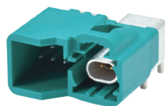
544 HMTD-N 1x1 +MQS 6Pin R/A Type Coding: A,B,C,D,E,F,G,H,J,K,L,M,O,Z Positions: 06+02
