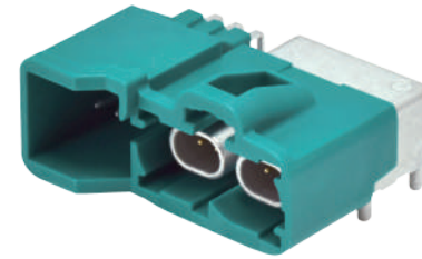
144 HMTD-N 1x2 +MQS 6Pin R/A Type Coding: A,B,C,D,E,F,G,H,J,K,L,M,O,Z Positions: 06+04
