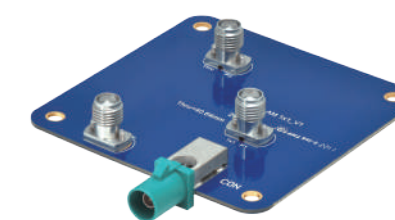
Calibration Jig FAKRA Plug R/A Middle Type, CH=0.33 Coding: A,B,C,D,E,F,G,H,I,K,L,M,N,Z Positions: 01
