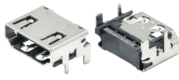
508 HDMI 2.1V Conn. Positions:19
