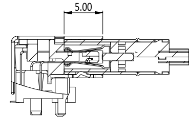
FULLY MATED MINI DISPLAYPORT CONNECTOR SHOWING MATING LEVELS
