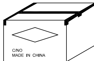
(CARTON:L17.75"*W12.5"*H13",Material K=K) (25PCS CABLE/CARTON)
