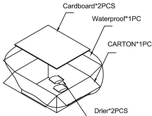
(CARTON:L17.75"*W12.5"*H13",Material K=K) (25PCS CABLE/CARTON)
