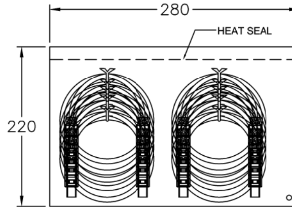
PE BAG:L280*W220*T0.05mm 10PCS CABLE/PE BAG
