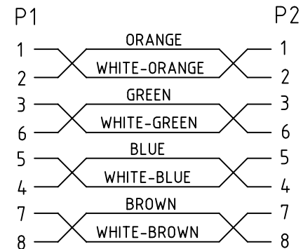
WIRE ARRANGEMENT
