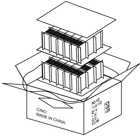
(包裝視圖)
