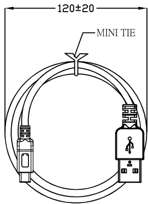
USB C/AM 2.0 CABLE
