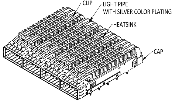
WITH HEATSINK, WITH LIGHT PIPES LIGHT PIPE WITH SILVER COLOR PLATING
