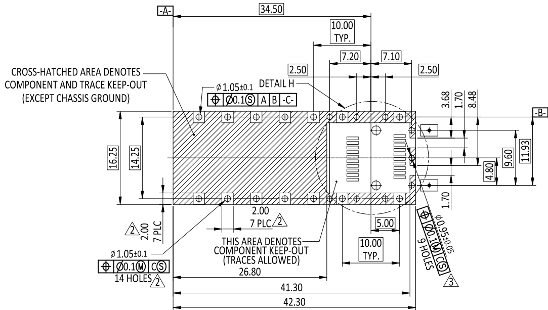
RECOMMENDED PCB CONFIGURATION WITH KEEP-OUT AREAS BELLY TO BELLY APPLICATIONS
