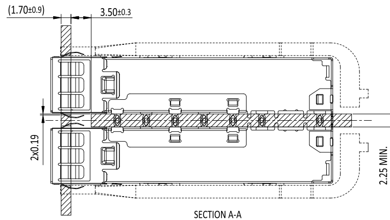
RECOMMENDED BEZEL DESIGN BELLY TO BELLY APPLICATIONS
