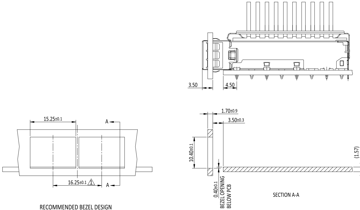
RECOMMENDED BEZEL DESIGN
