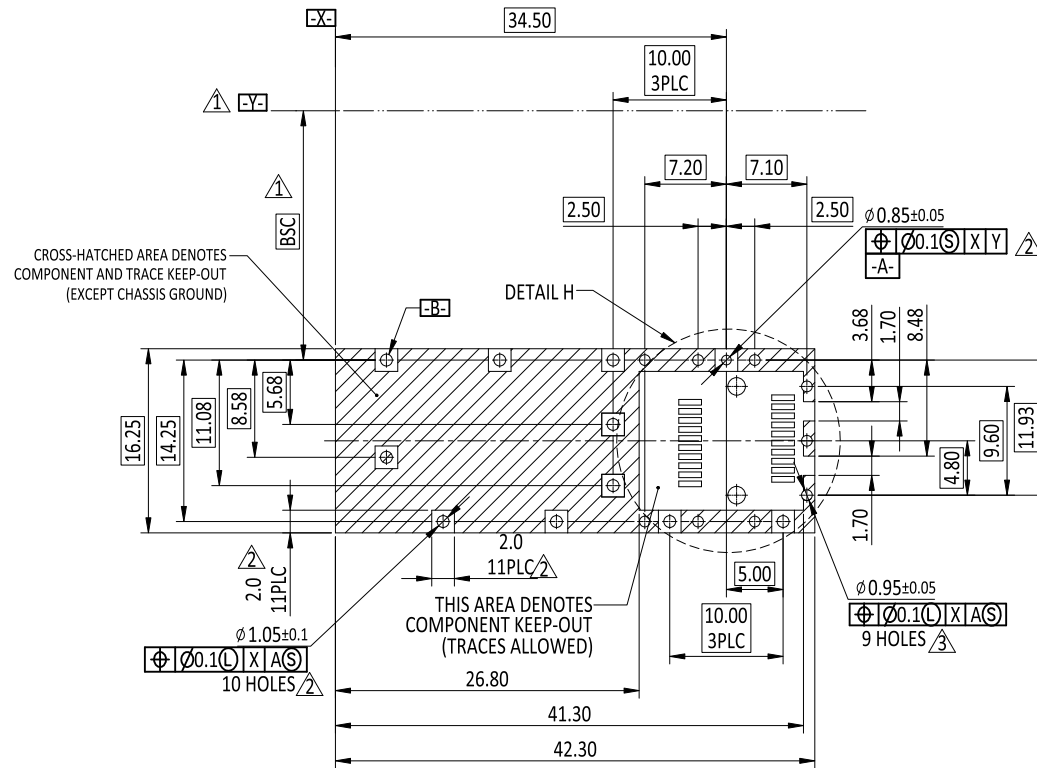
RECOMMENDED PCB CONFIGURATION
