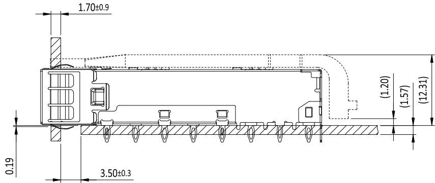
BEZEL OPENING BELOW PC BOARD
