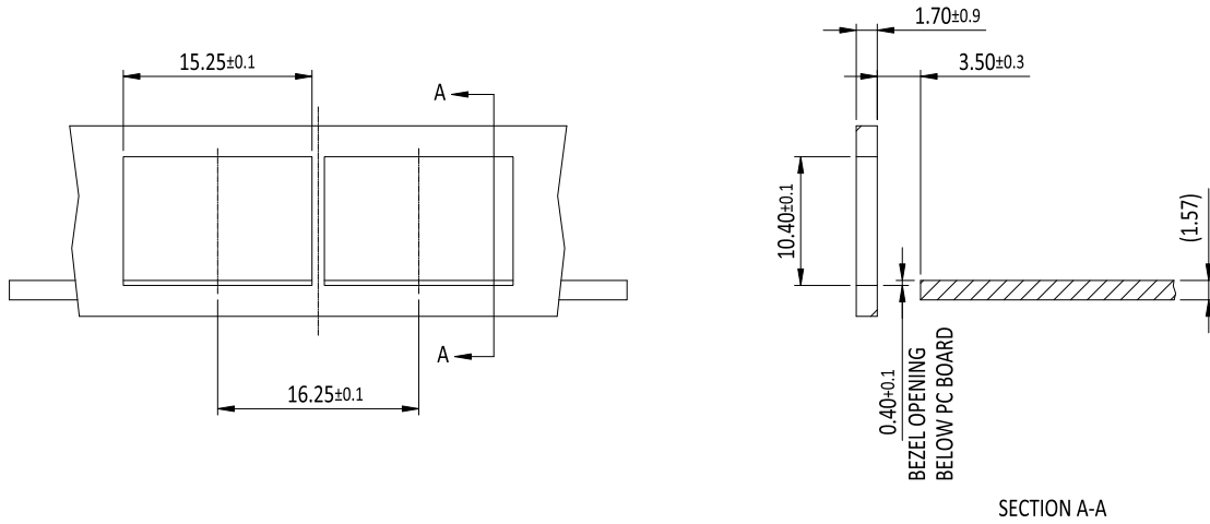
RECOMMENDED BEZEL DESIGN
