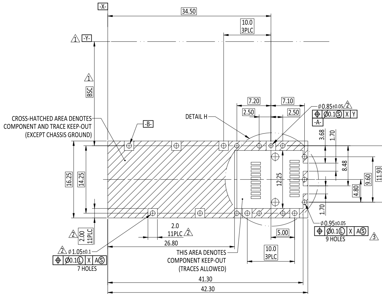
ECOMMENDED PCB CONFIGURATION
