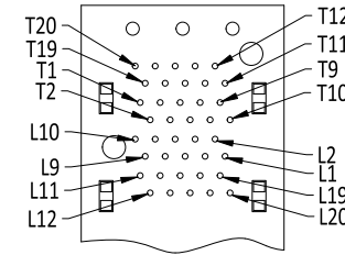
CONNECTOR PIN-OUT COMPONENT SIDE OF BOARD
