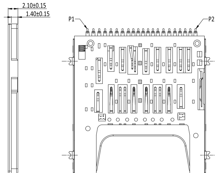
SD7.0 PUSH CARD CONN.
