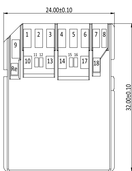
SD EXPRESS CARD
