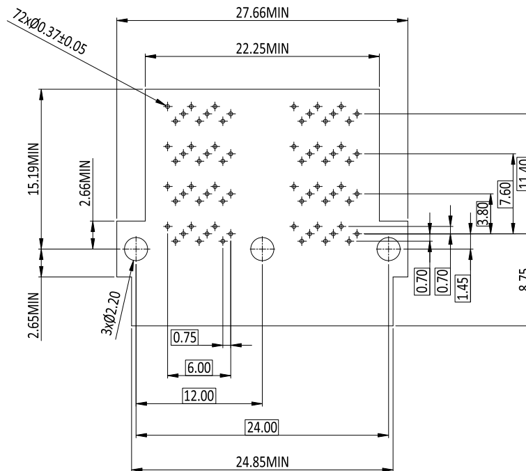
RECOMMENDED PCB LAYOUT(1x2)
