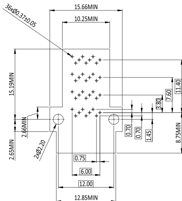
RECOMMENDED PCB LAYOUT(1x1)
