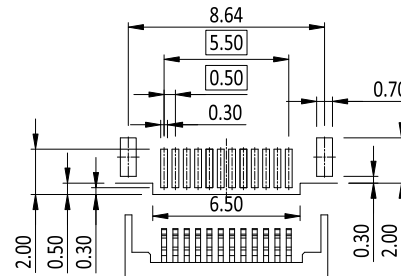
RECOMMENDED PCB LAYOUT (T: 1.00mm) TOLERANCE UNSPECIFIED ±0.05mm
