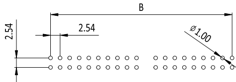
RECOMMENDED PCB HOLE LAYOUT
