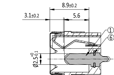
A'-A' SECTION
