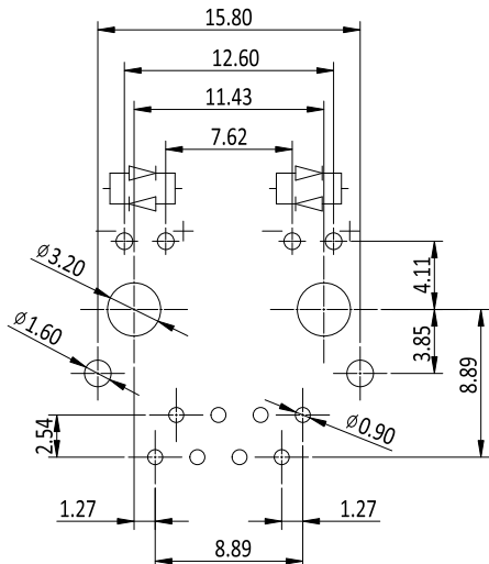
PCB LAYOUT (TOP VIEW) TOLERANCES: \pm 0.05\text{mm}
