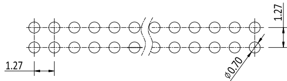
RECOMMENDED PCB LAYOUT (TOP SIDE) TOLERANCE±0.05
