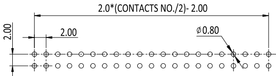
RECOMMENDED PCB HOLE LAYOUT
