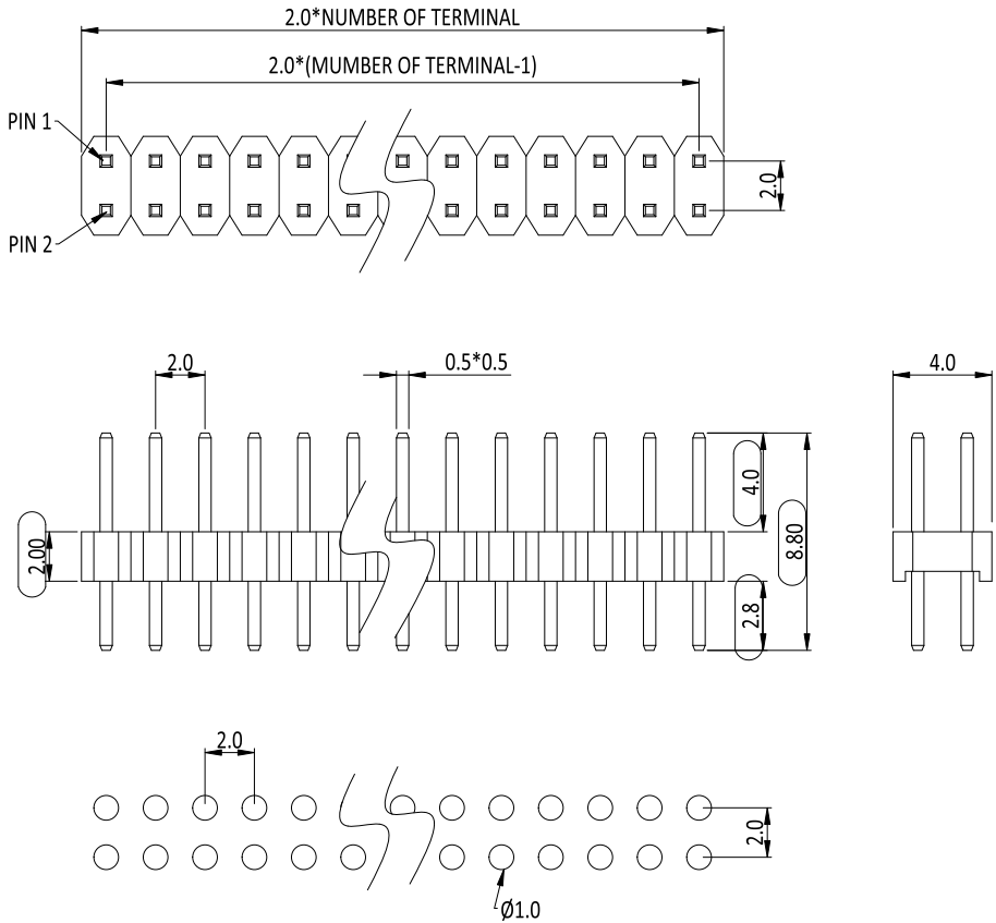
RECOMMENDED PCB LAYOUT(TOP VIEW) TOLERANCES: ±0.05mm
