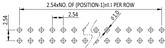
RECOMMENDED PCB LAYOUT(TOP VIEW) TOLERANCES: ±0.05mm
