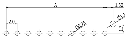
RECOMMENDED PCB LAYOUT(TOP VIEW) TOLERANCES: ±0.05mm
