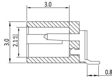
SECTION X-X
