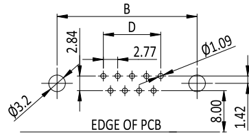
RECOMMENDED PCB LAYOUT (TOP VIEW) TOLERANCES: ±0.05mm
