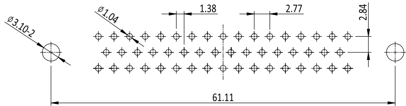
RECOMMEND PCB LAYOUT TOP VIEW
