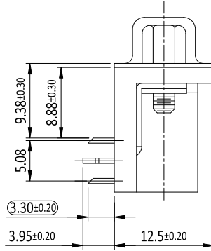
PARTS DIMENSION TABLE
