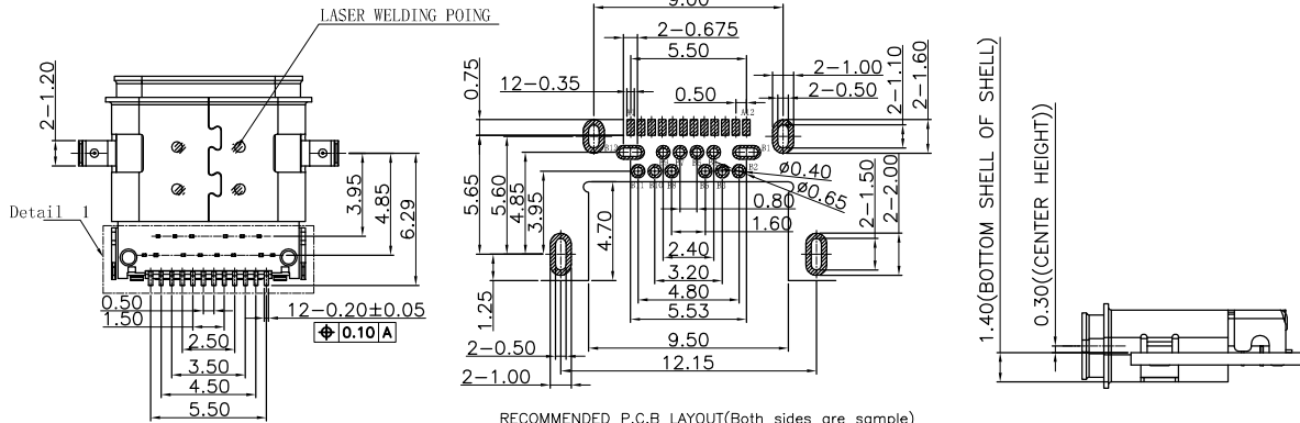
RECOMMENDED P.C.B LAYOUT(Both sides are sample) Tolerance:±0.05, Thickness=0.60mm
