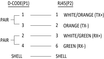
WIRING DIAGRAM(26AWG)
