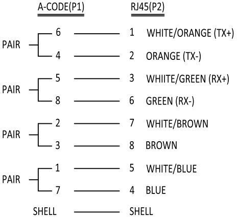
WIRING DIAGRAM
