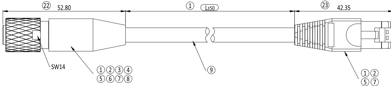
WIRING DIAGRAM(26AWG)
