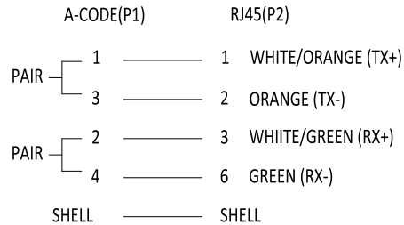
WIRING DIAGRAM(26AWG)
