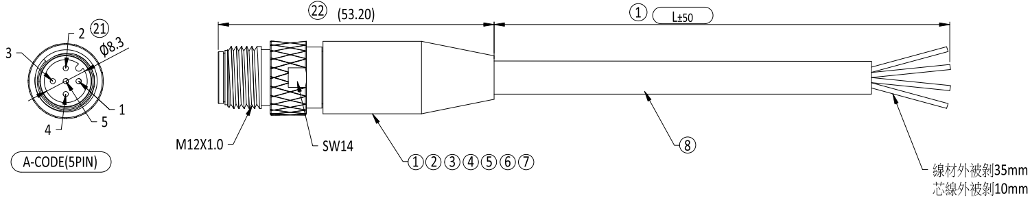
WIRING DIAGRAM(22AWG)
