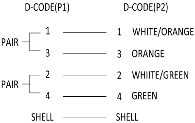
WIRING DIAGRAM(26AWG)
