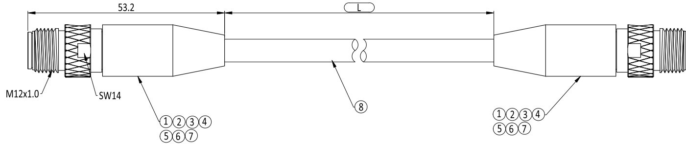
WIRING DIAGRAM(26AWG)
