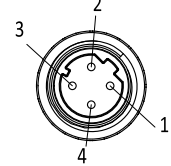
WIRING DIAGRAM(26AWG)
