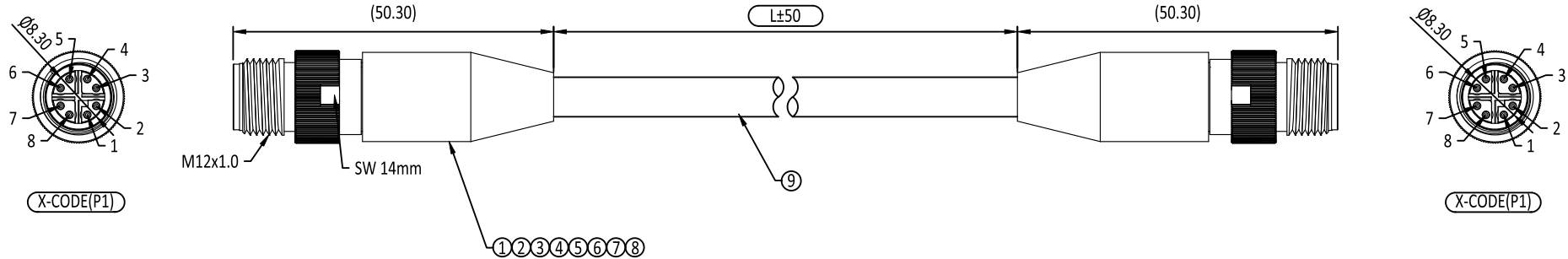
WIRING DIAGRAM
