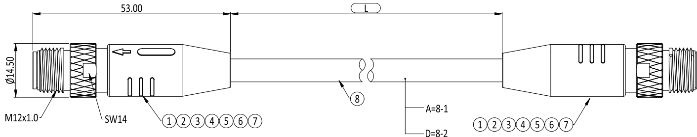
WIRING DIAGRAM(A-CODE 22AWG)
