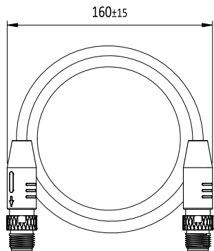
M12 CABLE
