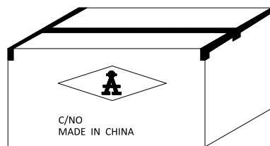
CARTON: L457xW298xH228mm, MATERIAL K=K
