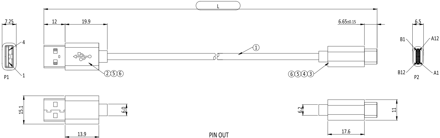
PIN OUT
