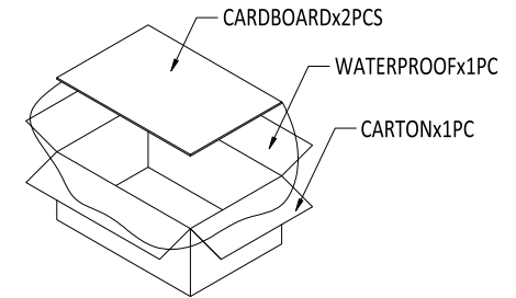
(CARTON: L457xW298xH228mm, MATERIAL K=K)
