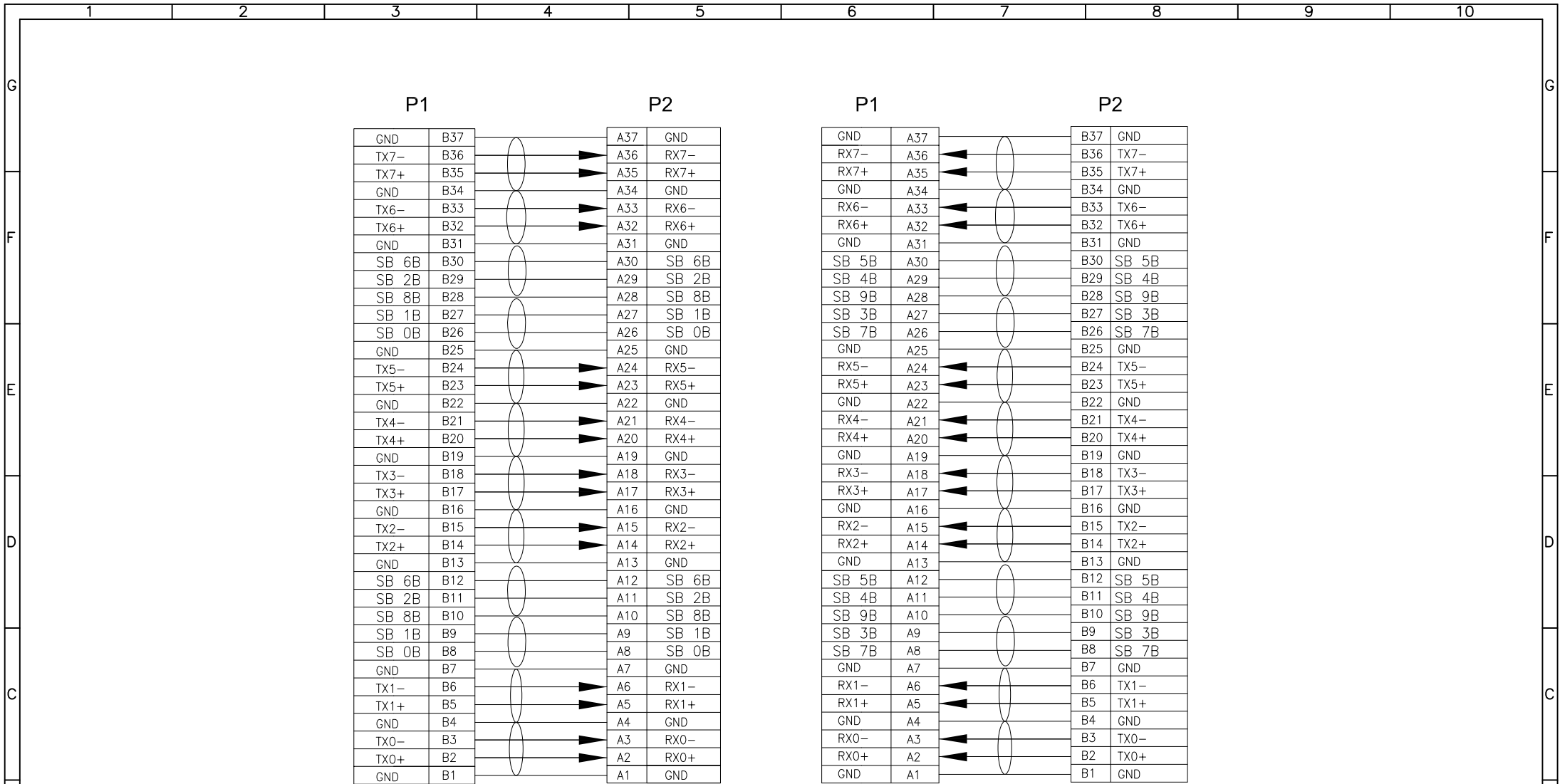
WIRE DIAGRAM
