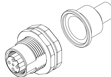
M12 CONN. RIVETING METAL SR
