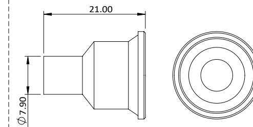
PARTS DIMENSION TABLE: METAL SR
