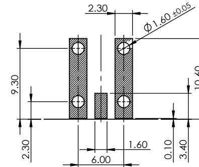
RECOMMENDED P.C.B. LAYOUT TOLERANCE : ±0.02mm
