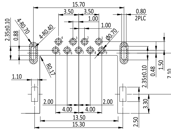
RECOMMENDED PCB LAYOUT TOLERANCES: ±0.05mm
