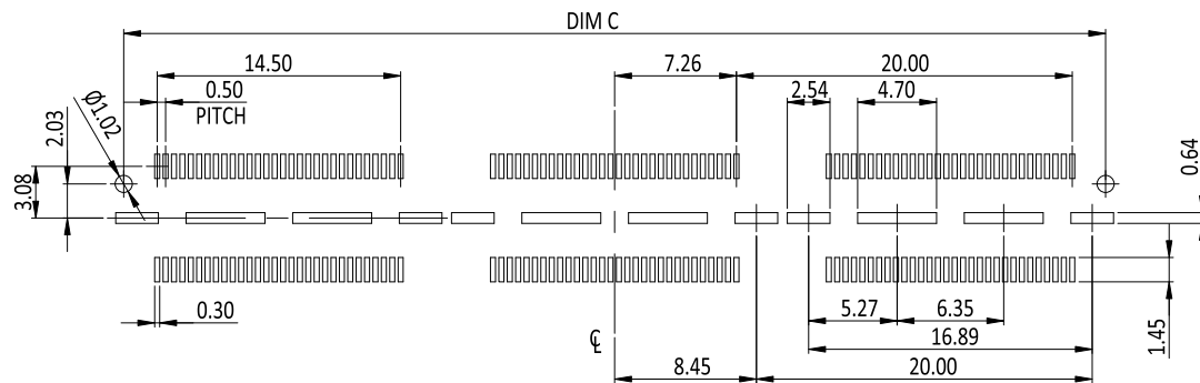
RECOMMENDED PCB LAYOUT TOLERANCES:±0.03mm
