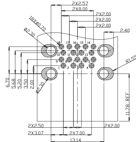
RECOMMENDED P.C.B LAYOUT TOLERANCES:±0.05mm
