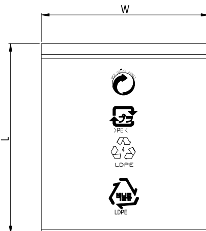
ZIP BAG: 203(L)x165(W)x0.05(T)mm
